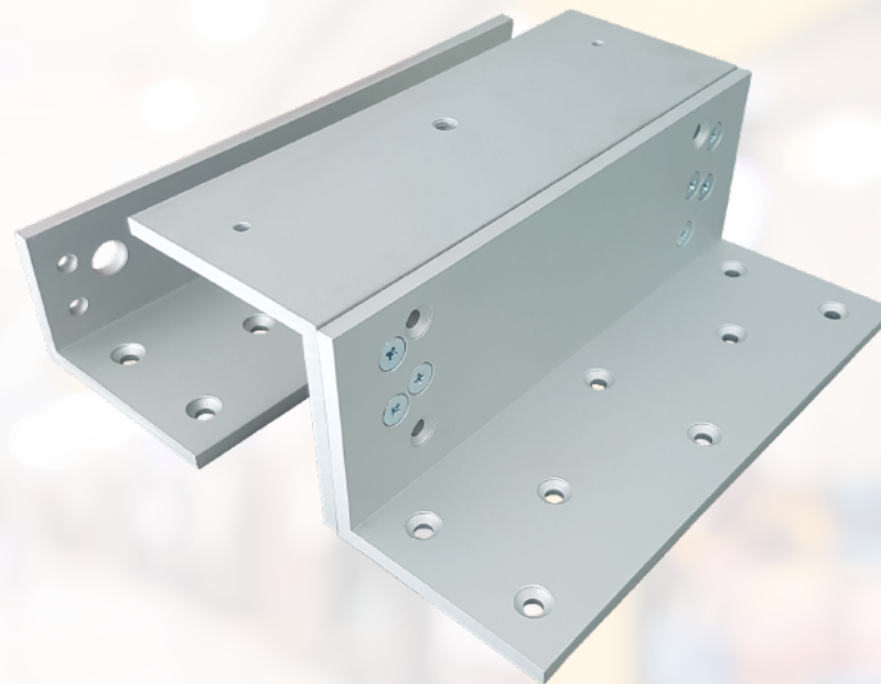
VIS-ZL-SS1500-G L and Z Bracket for VIS-SS1500-G Outdoor 1500lbs Maglock
