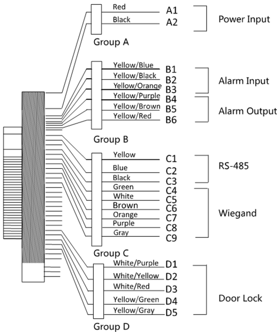
Figure 4-1 Terminal Diagram
