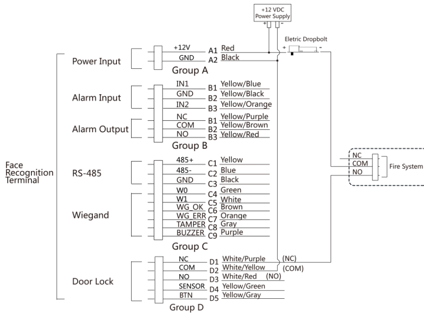
Figure 4-6 Wiring Device
