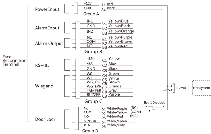
Figure 4-4 Wire Device
