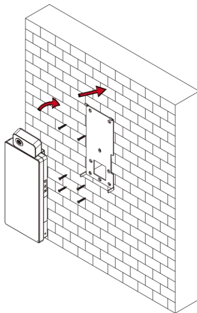
Figure 3-6 Install Device
