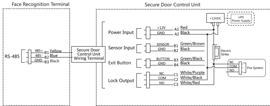
Figure 4-9 Wiring Diagram
