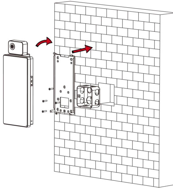
Figure 3-2 Install Device
