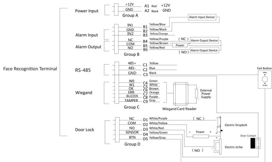
Figure 4-2 Device Wiring
