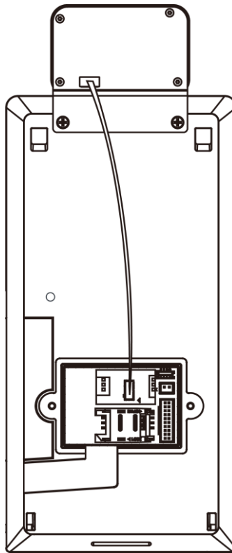
Figure 3-1 Connect Thermographic Module
