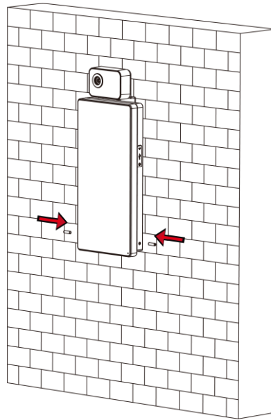
Figure 3-3 Secure Device
