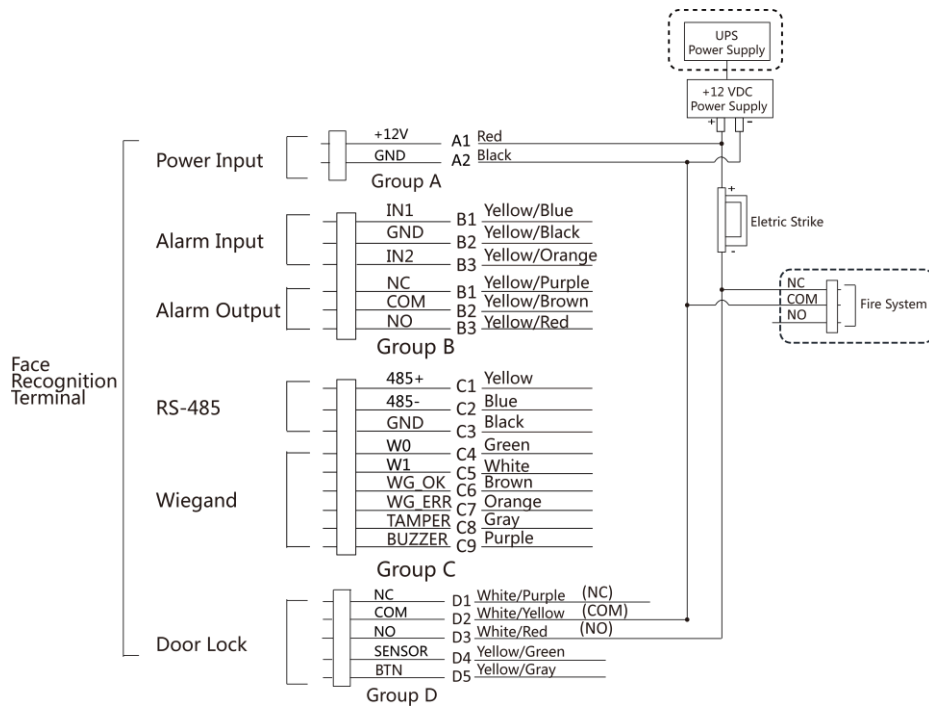
Figure 4-8 Device Wiring
