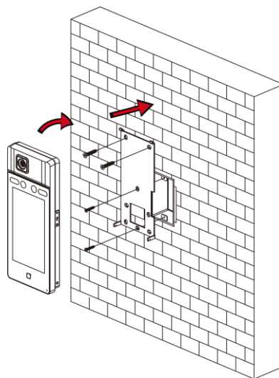
Figure 3-1 Install Device
