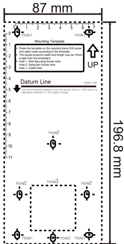
Figure 3-3 Mounting Template
