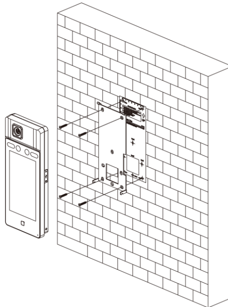
Figure 3-6 Install Device
