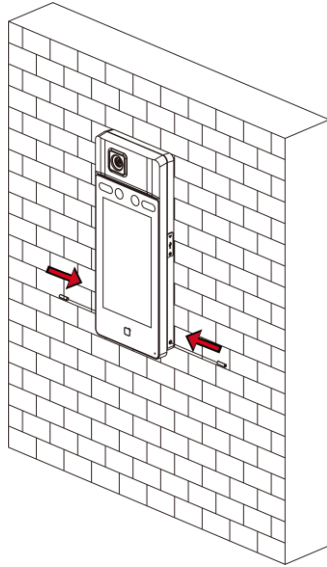
Figure 3-2 Secure Device
