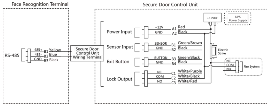
Figure 4-9 Wiring Diagram
