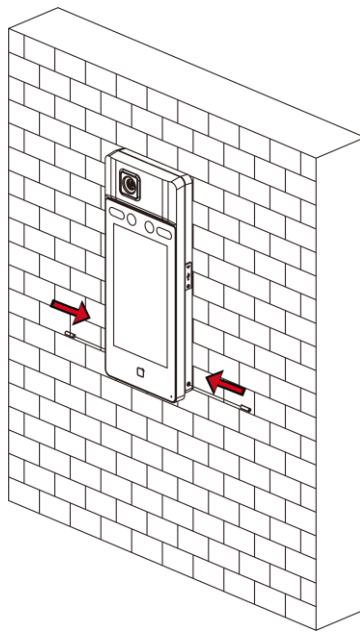
Figure 3-7 Secure Device
